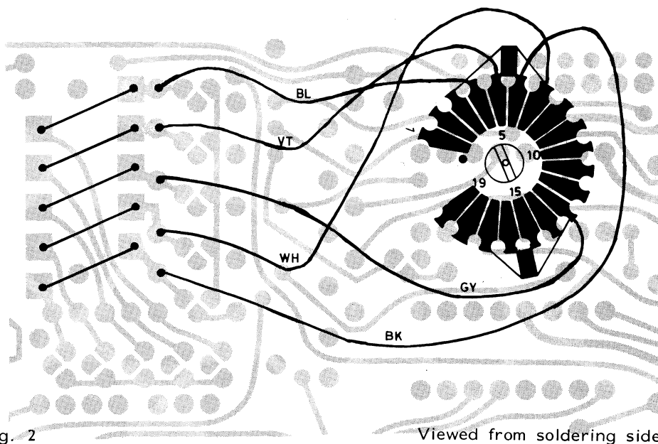
Part of printed circuit
