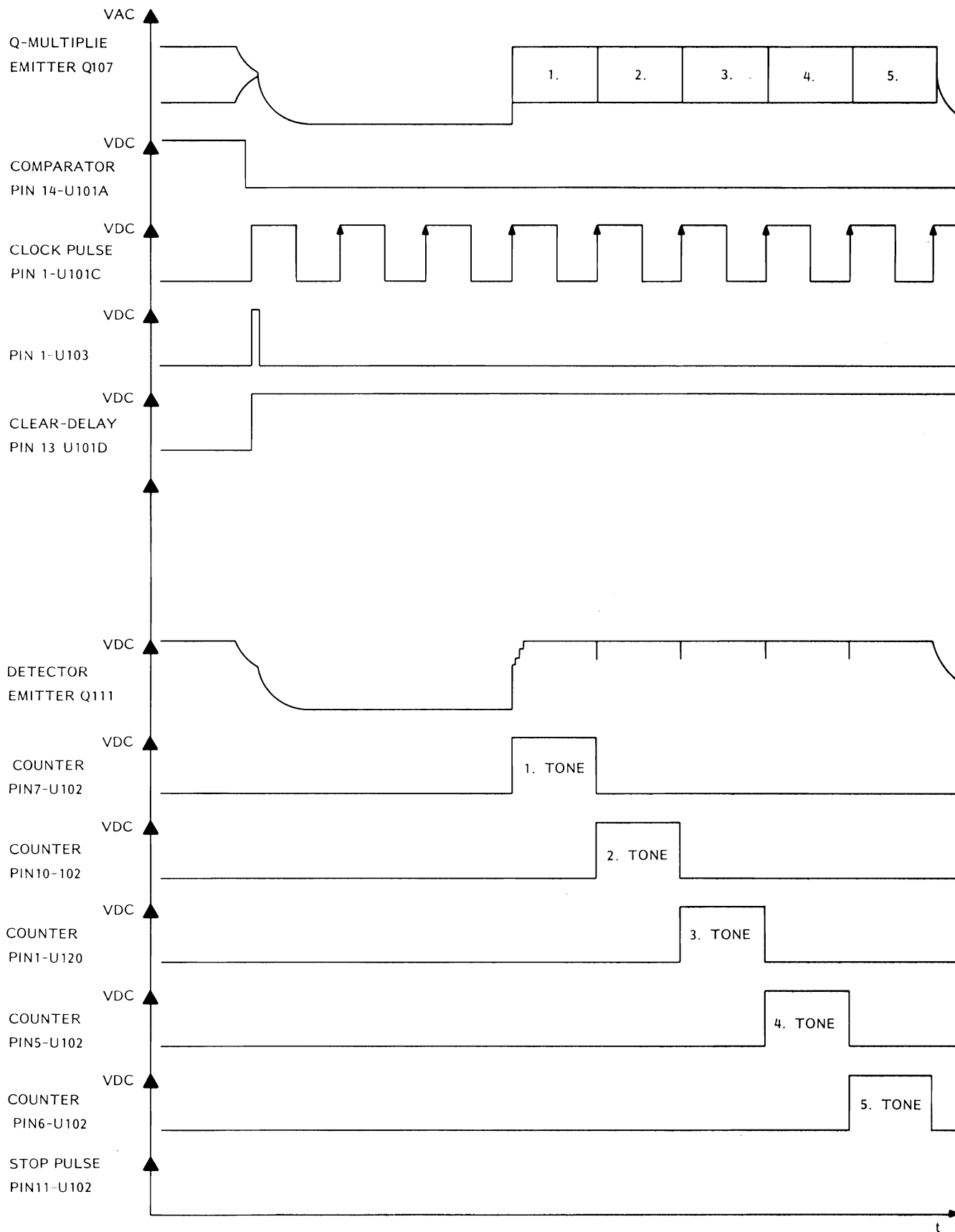
PULSE-TIME DIAGRAM FOR 5-TONE AUTOMATIC RECEIPT
